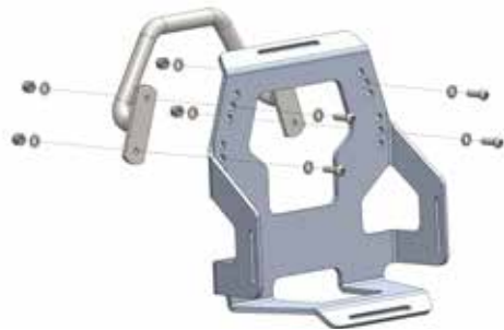
Mounting on C-Bow basic holder
